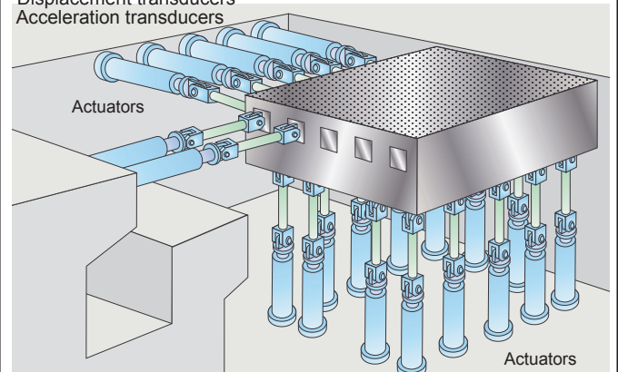
Real size 3D shaking table
